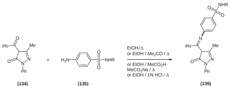
Scheme 36
