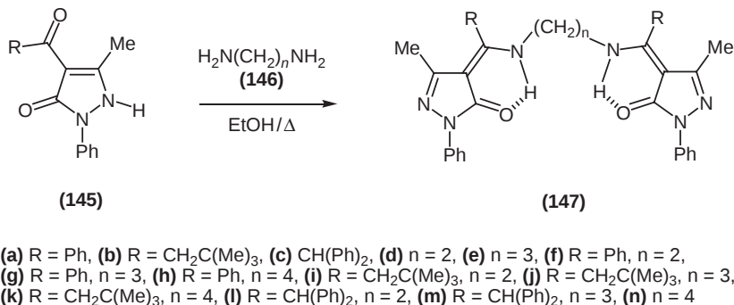
Scheme 39
