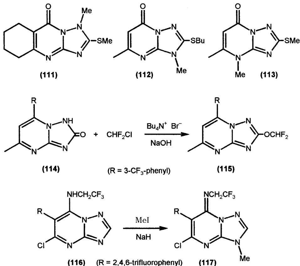
Scheme 30
