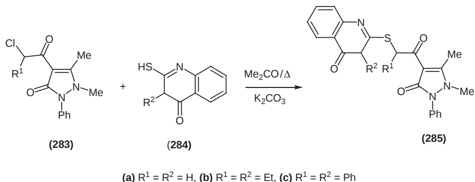
Scheme 76
