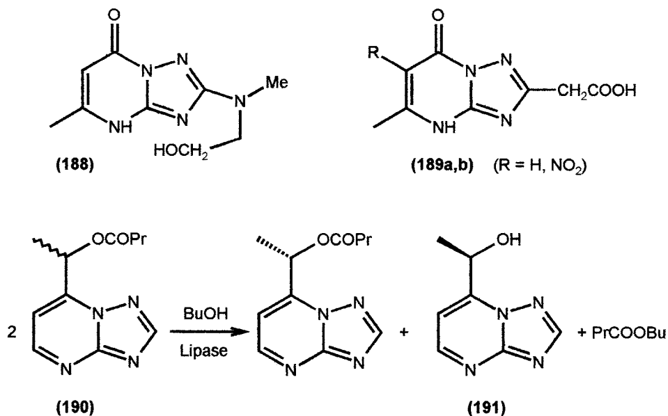
Scheme 48
