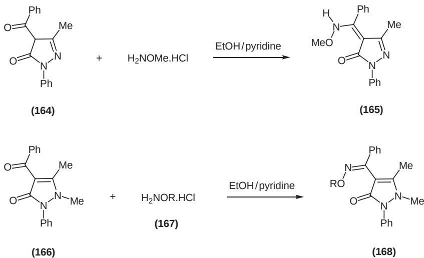
Scheme 43
