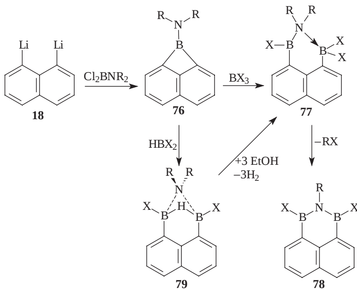
Scheme 15
