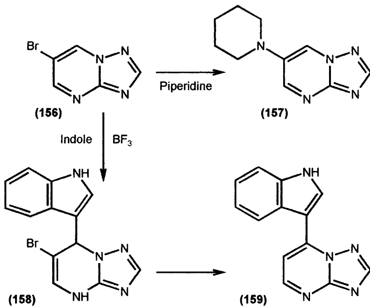
Scheme 40
