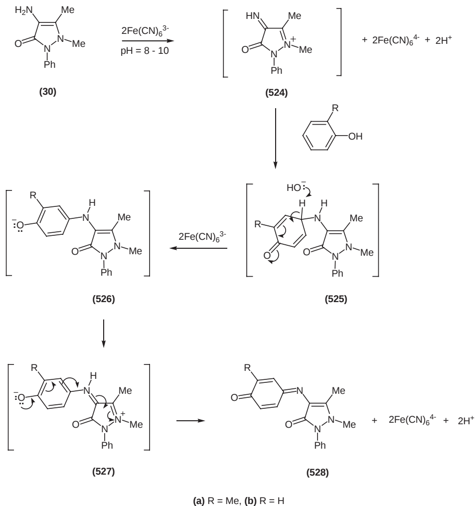
Scheme 144
