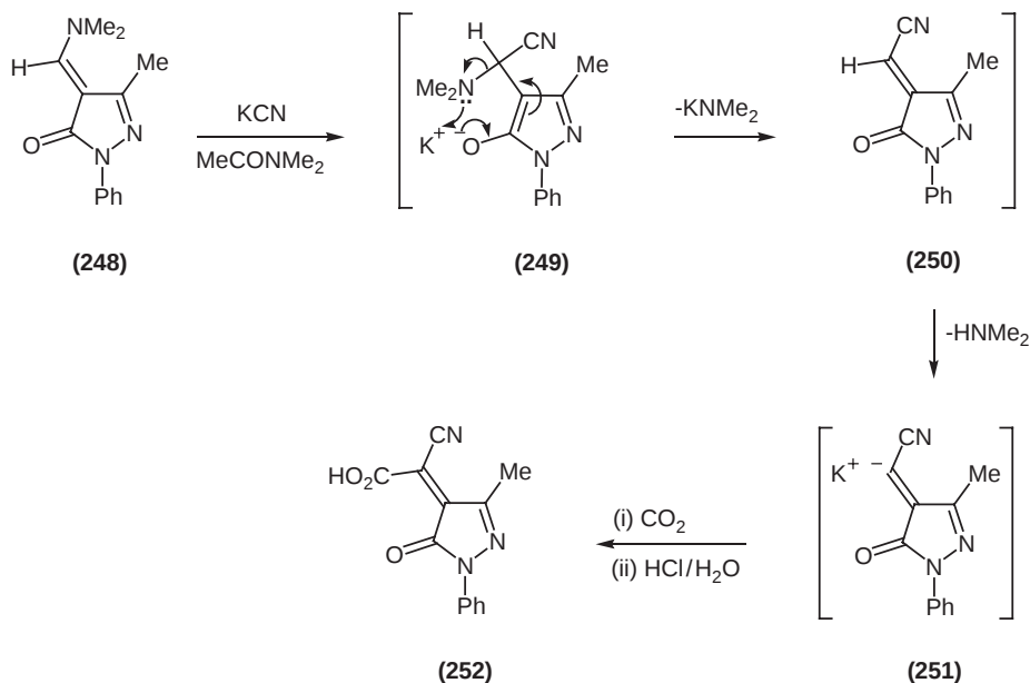
Scheme 67
