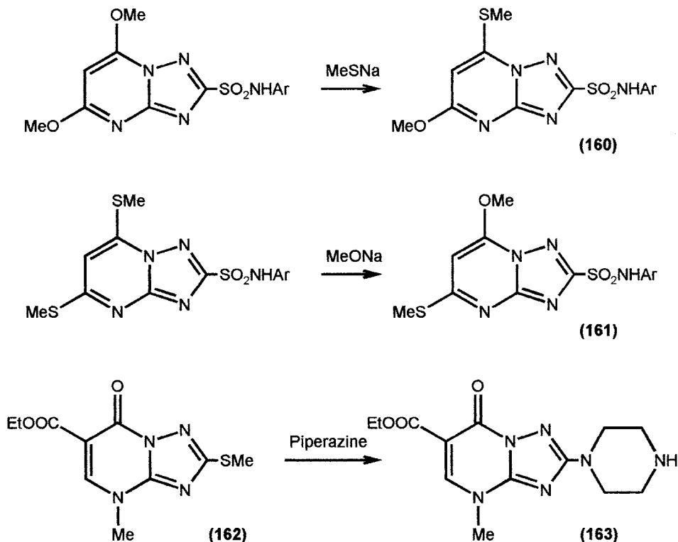
Scheme 41
