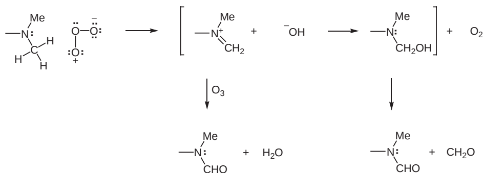
Scheme 139
