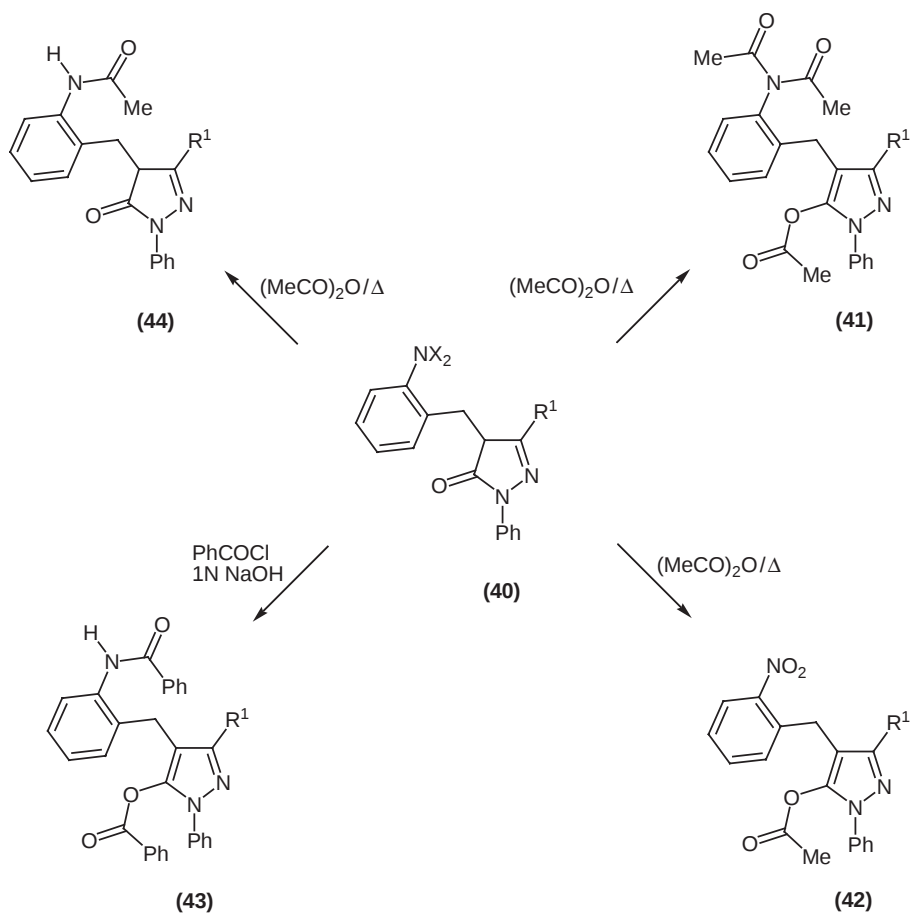
Scheme 9
