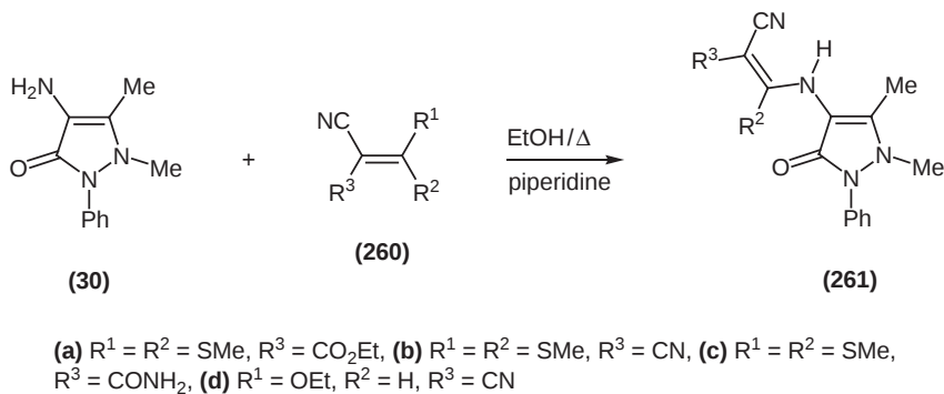
Scheme 70
