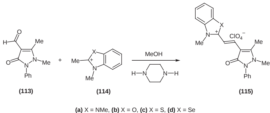
Scheme 32
