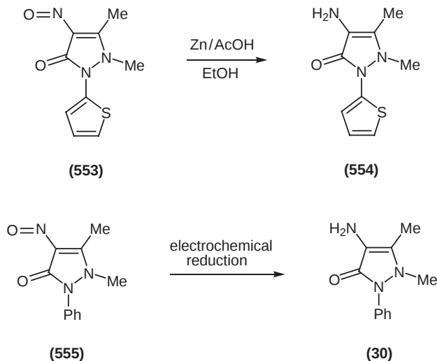
Scheme 153
