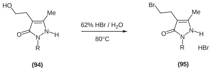
Scheme 26
