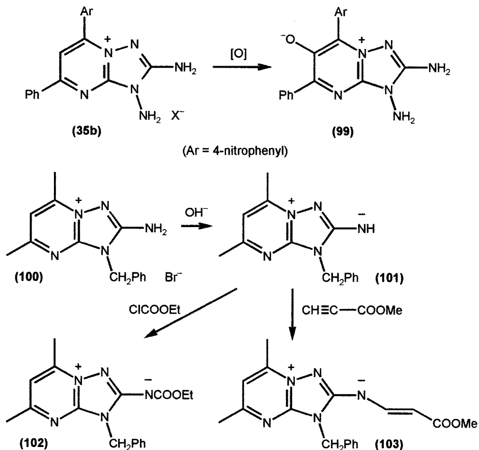
Scheme 27
