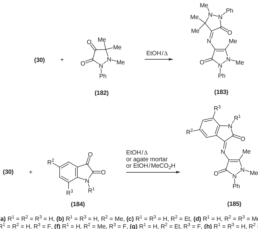
Scheme 48
