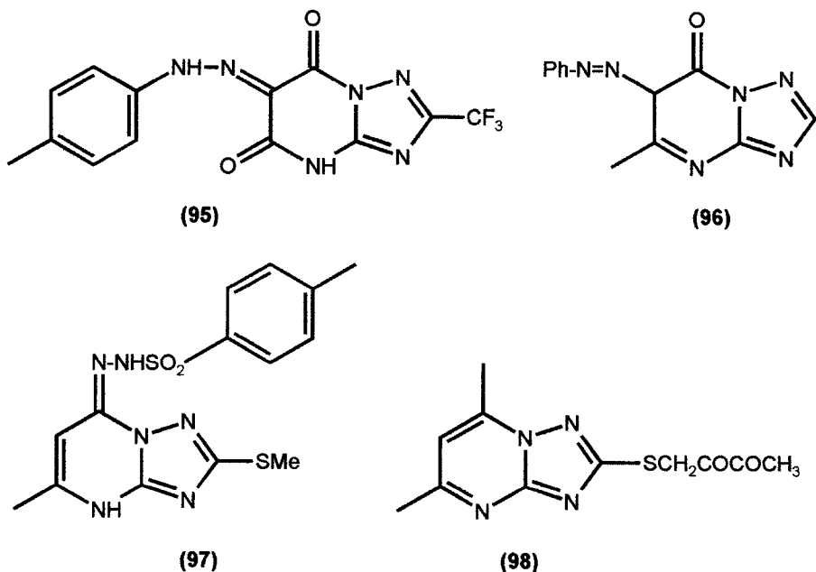
Scheme 26
