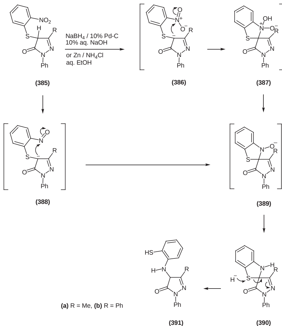
Scheme 108
