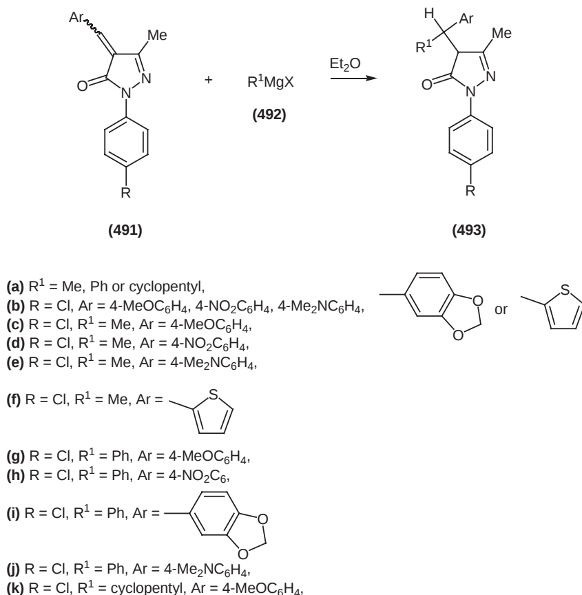
Scheme 133
