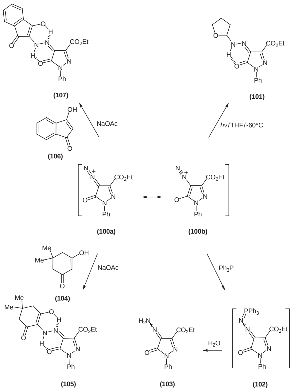
Scheme 29
