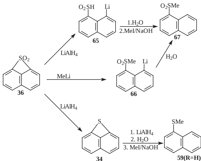
Scheme 11
