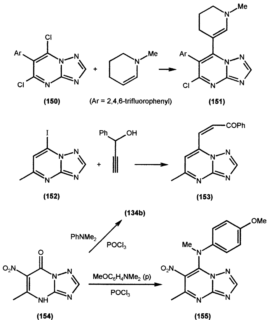
Scheme 39
