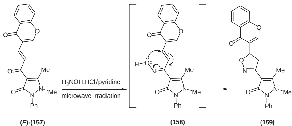
Scheme 42
