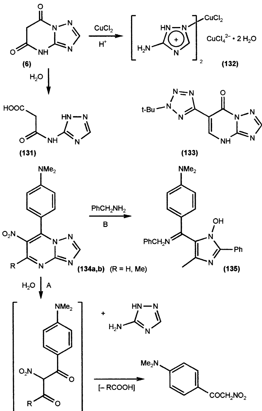
Scheme 34
