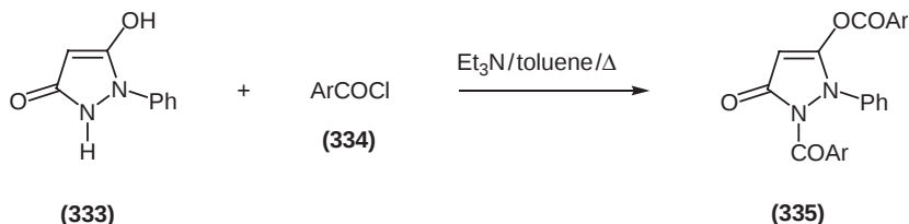
Scheme 91
