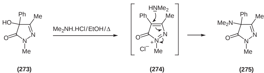
Scheme 73
