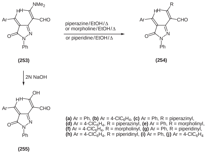
Scheme 68
