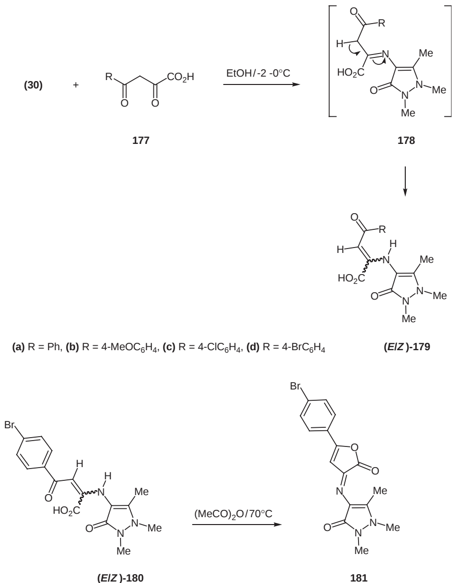
Scheme 47
