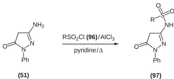
Scheme 27
