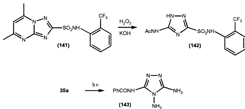
Scheme 36
