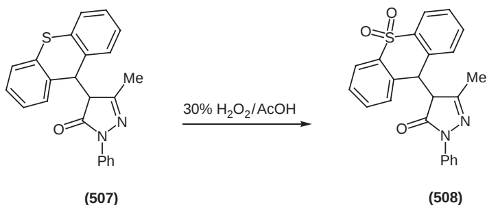
Scheme 140
