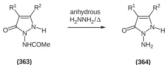
Scheme 99
