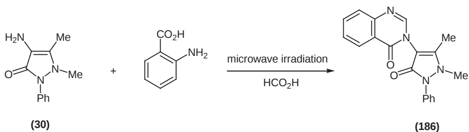
Scheme 49
