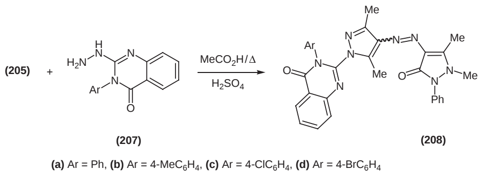
Scheme 55
