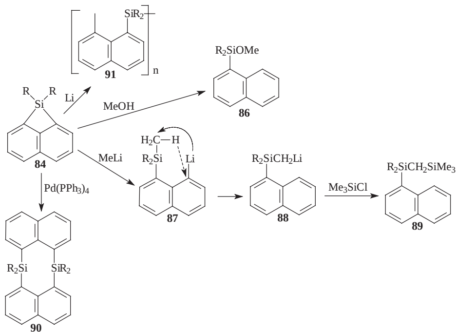
Scheme 19
