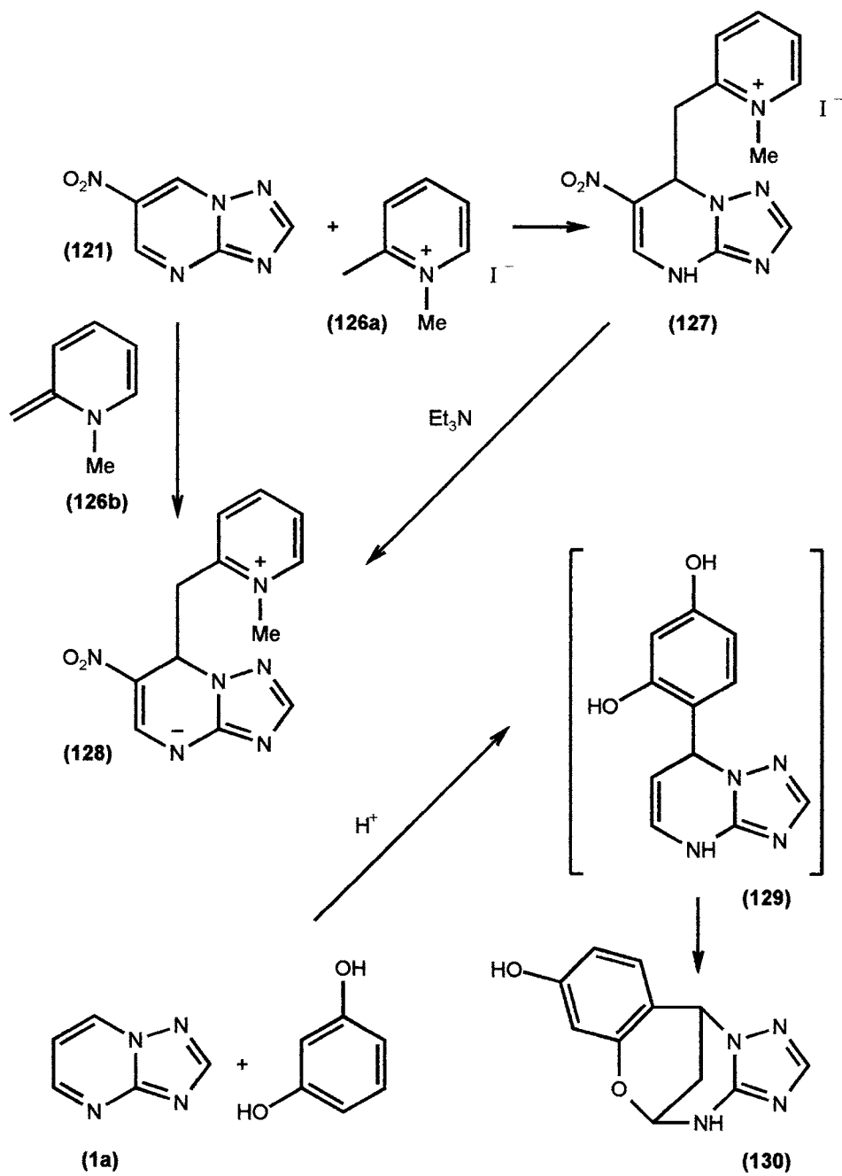
Scheme 33
