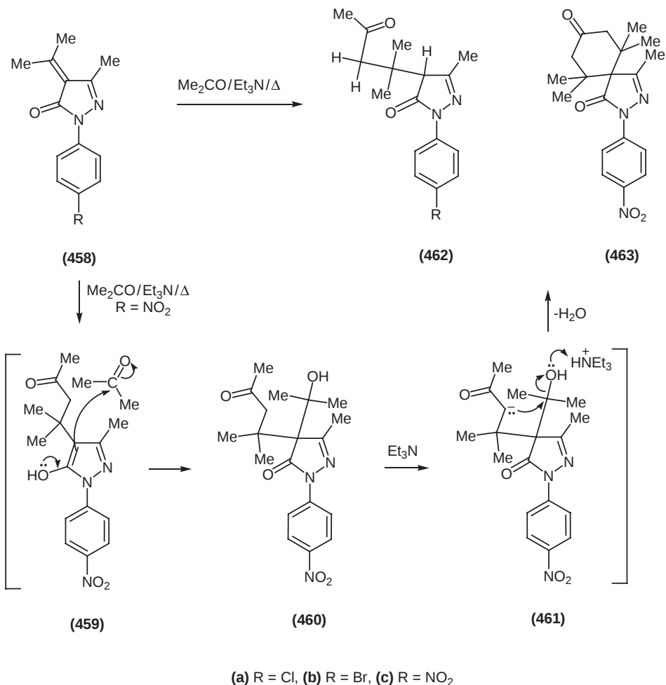
Scheme 126
