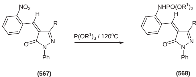
Scheme 159
