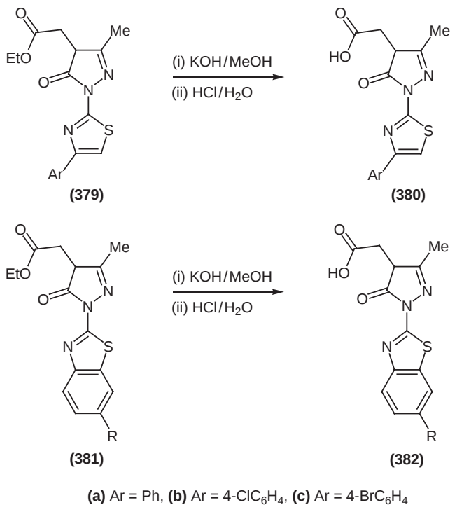
Scheme 106
