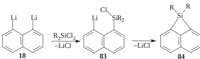
Scheme 17
