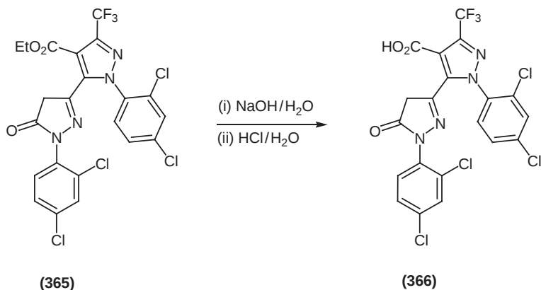
Scheme 101
