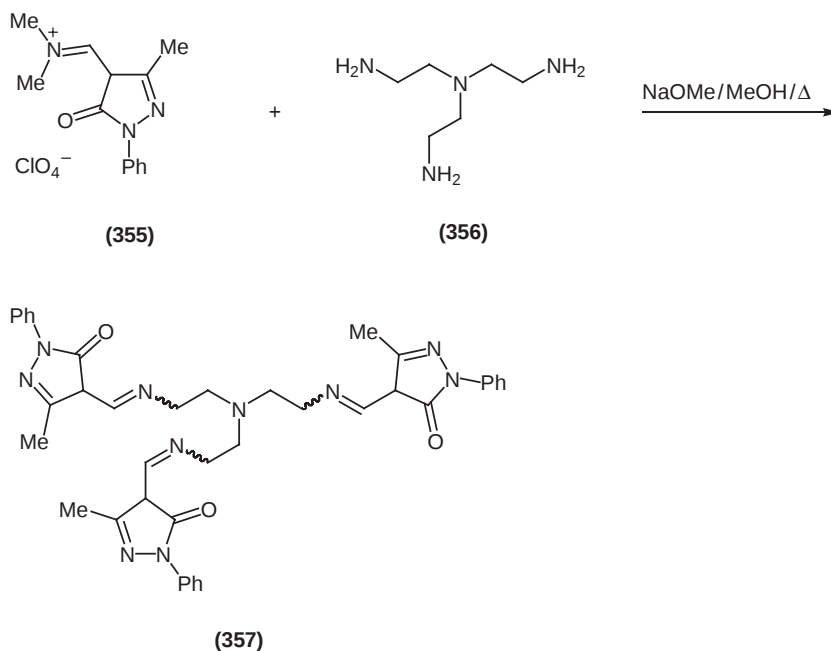
Scheme 97
