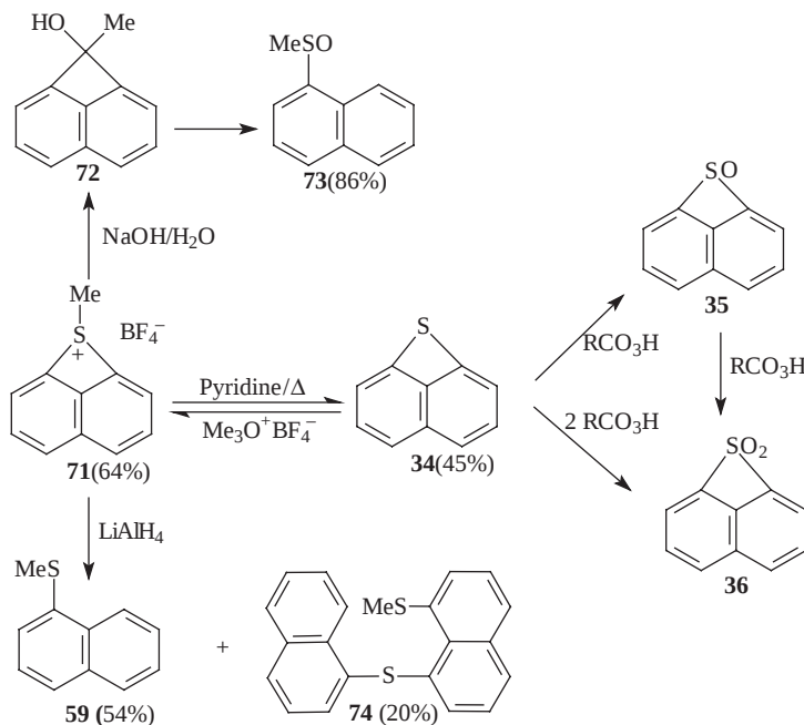
Scheme 14
