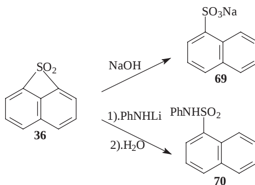
Scheme 13
