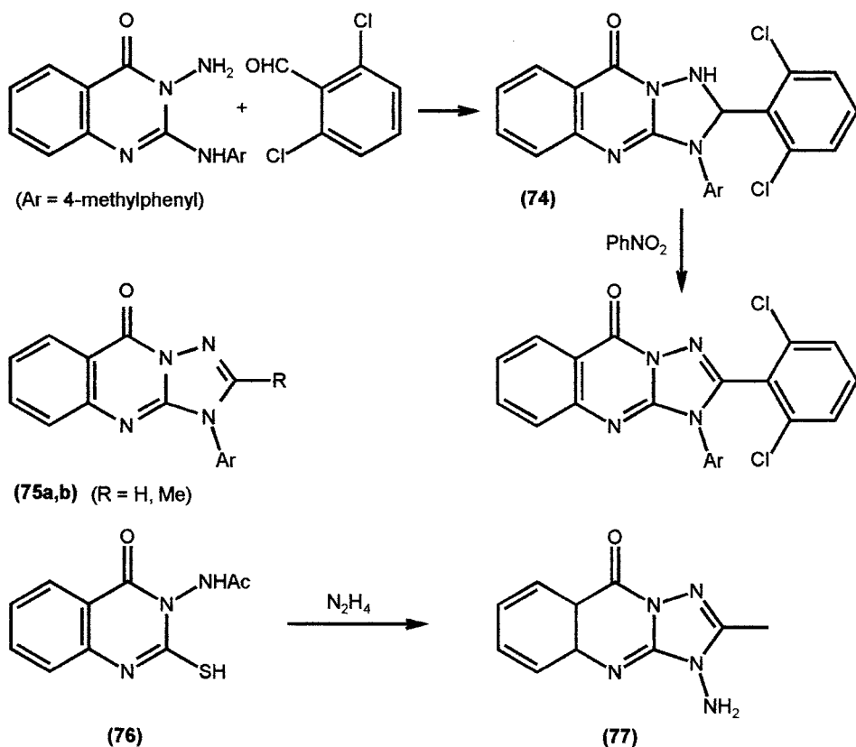
Scheme 19
