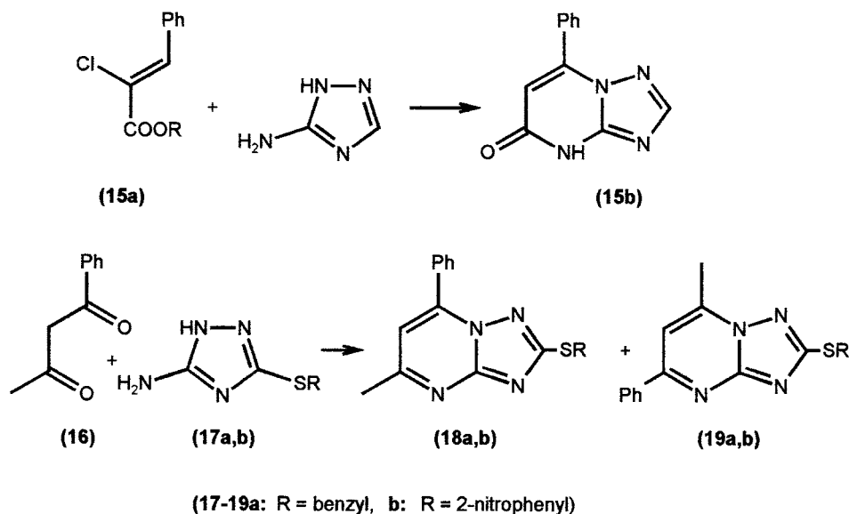
Scheme 6
