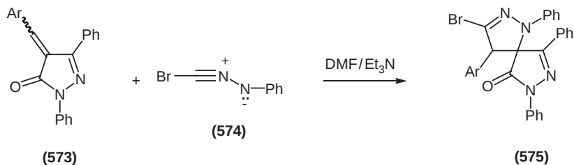
Scheme 160
