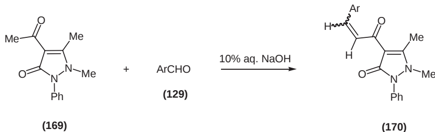
Scheme 44
