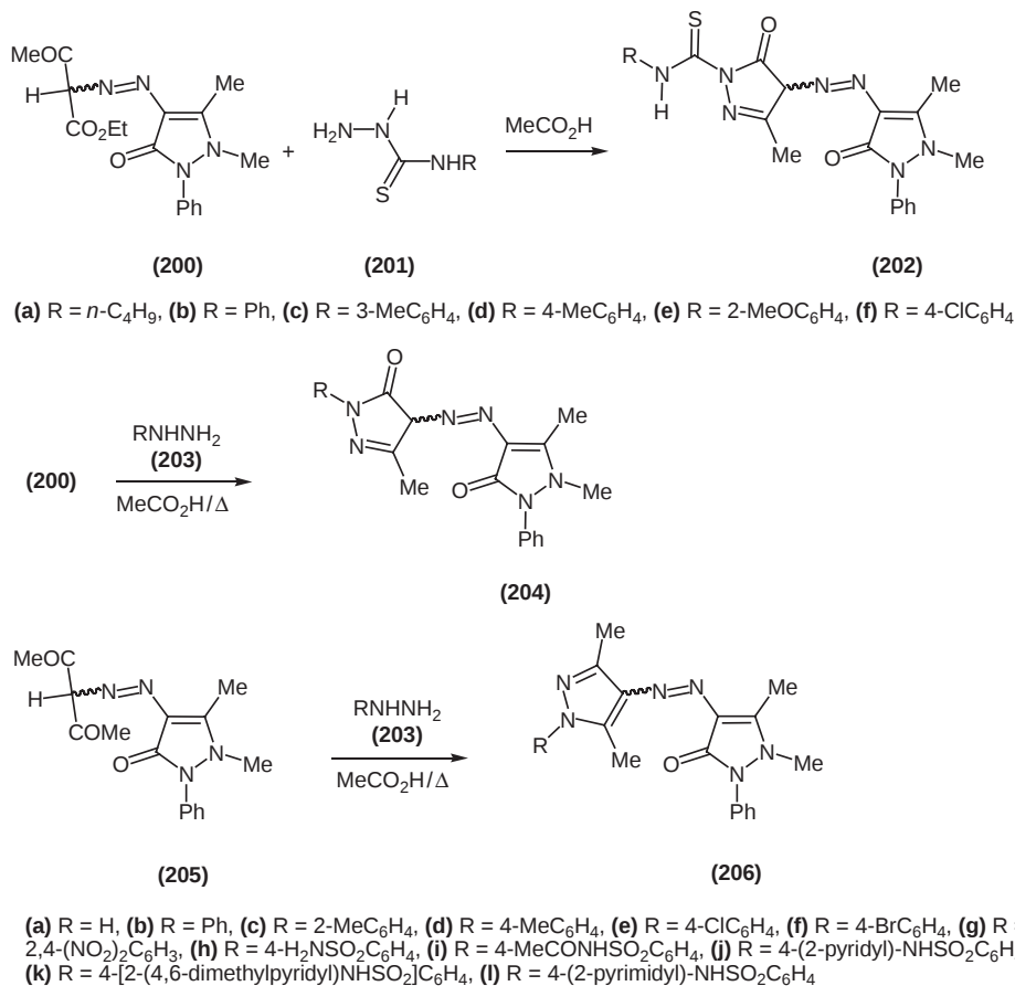
Scheme 54
