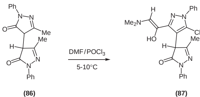
Scheme 22
