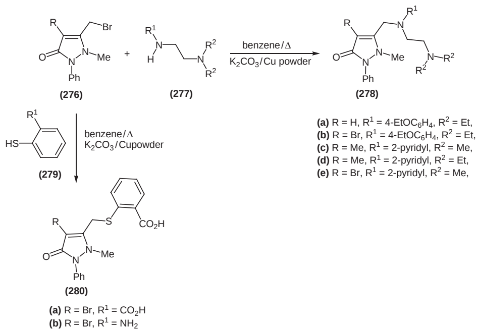
Scheme 74
