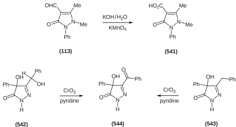
Scheme 149
