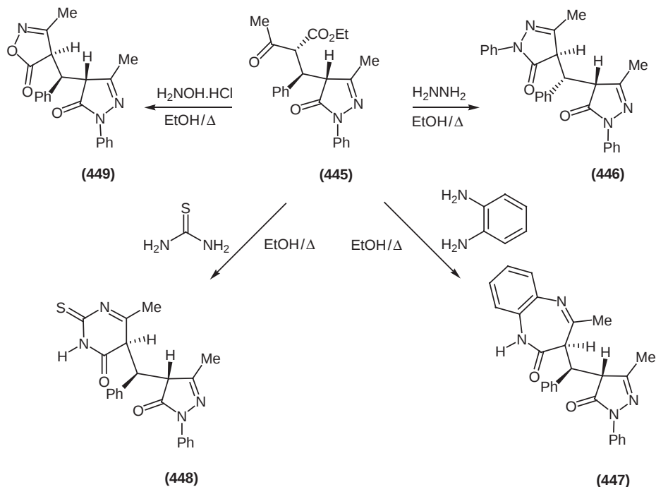
Scheme 123
