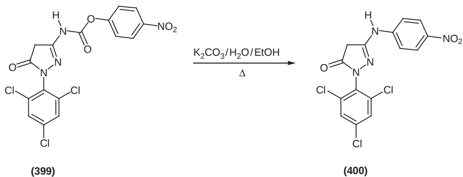
Scheme 110
