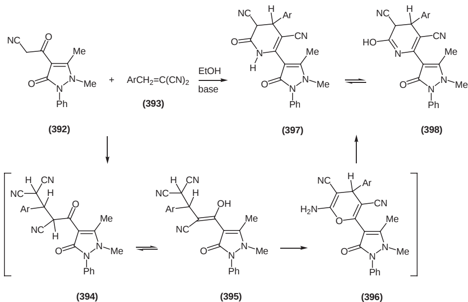
Scheme 109
