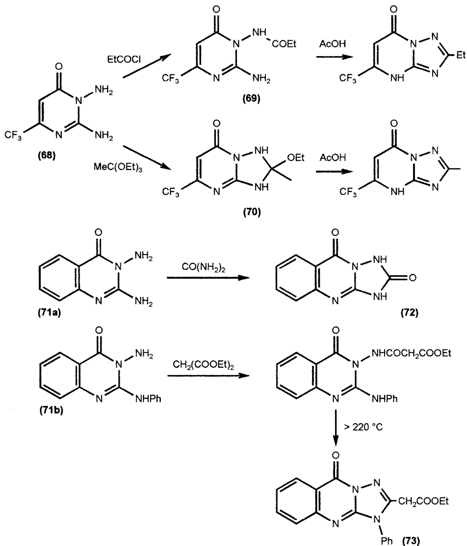
Scheme 18
