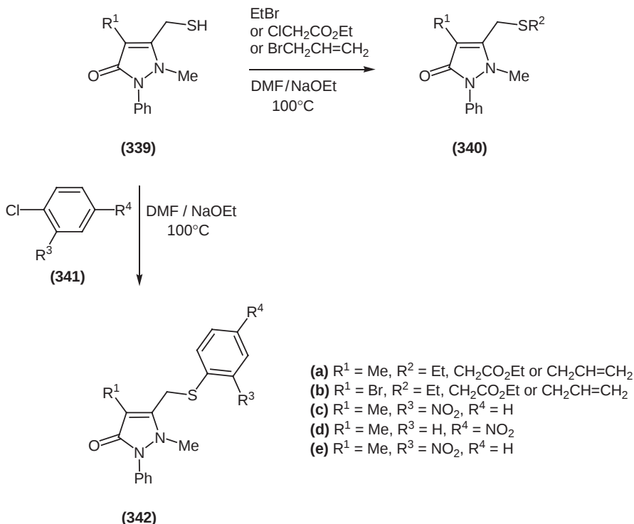
Scheme 93
