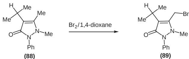
Scheme 23
