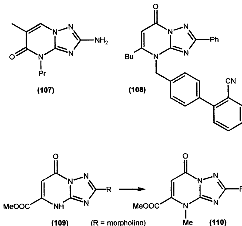
Scheme 29
