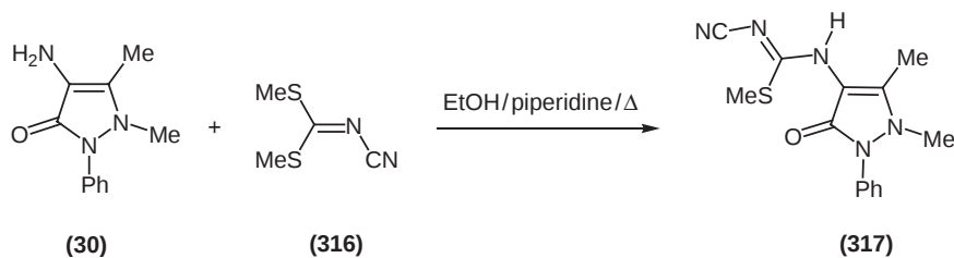
Scheme 86
