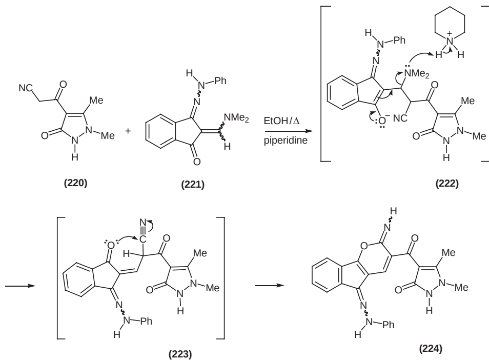
Scheme 59
