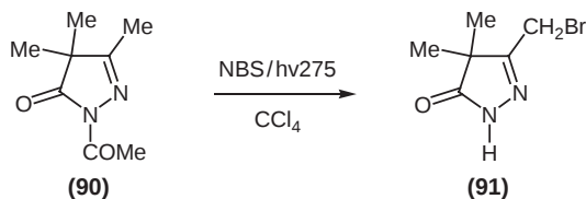
Scheme 24
