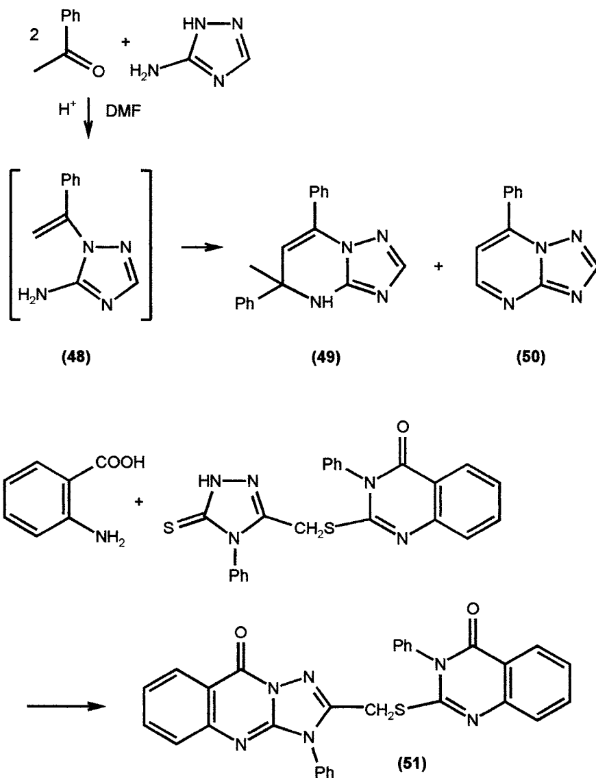
Scheme 13
