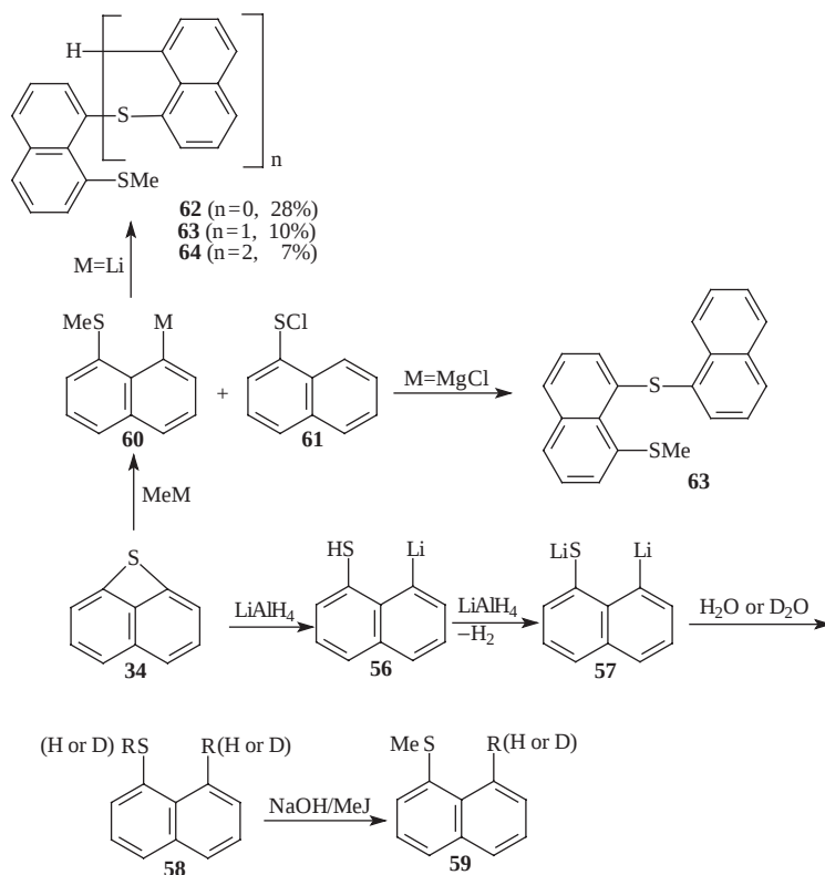
Scheme 10
