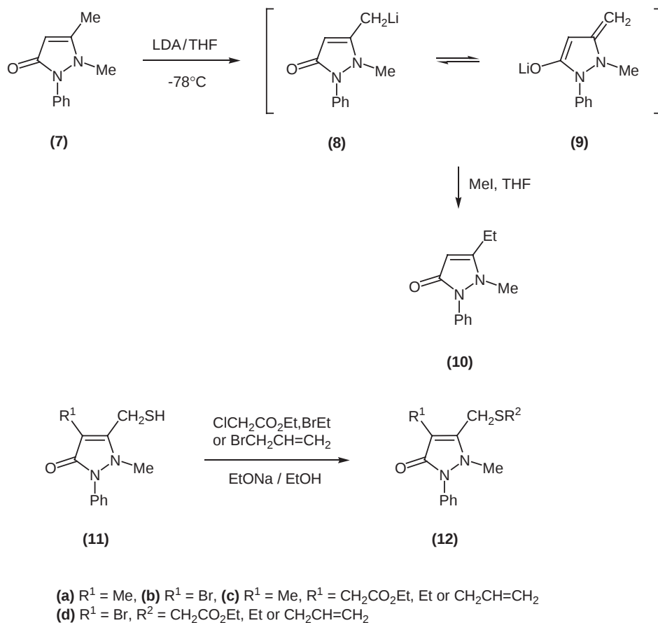
Scheme 2
