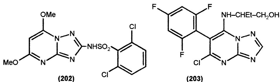
Scheme 52
