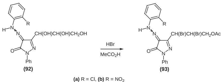
Scheme 25
