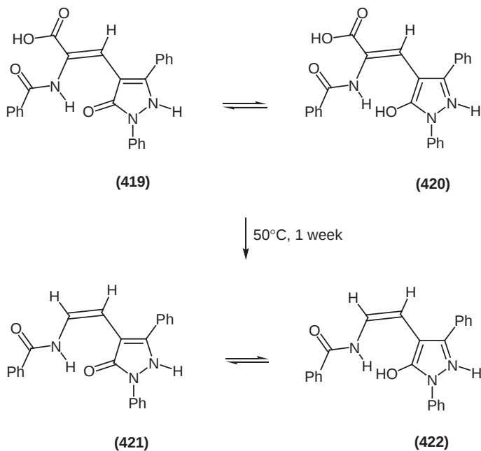
Scheme 116
