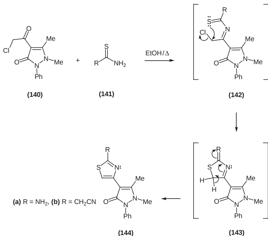
Scheme 38
