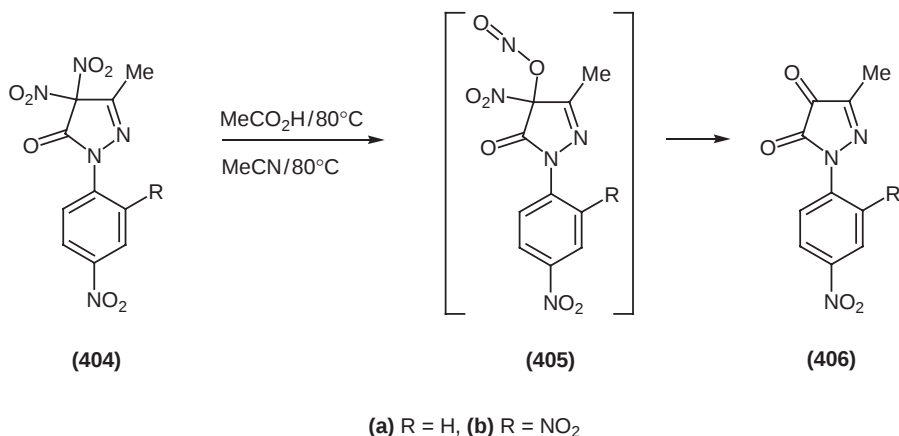
Scheme 112
