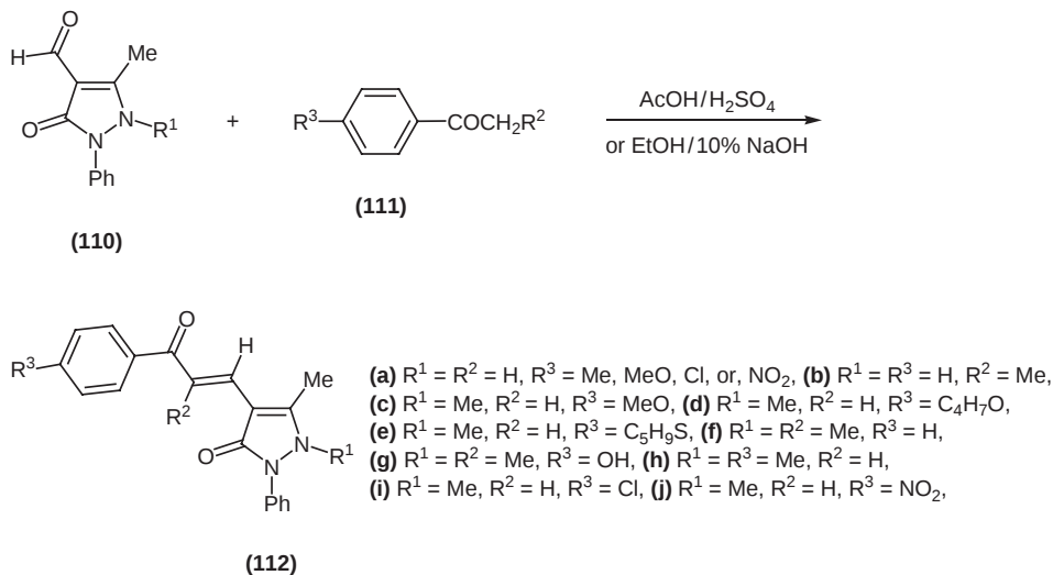
Scheme 31
