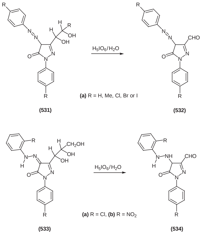
Scheme 146
