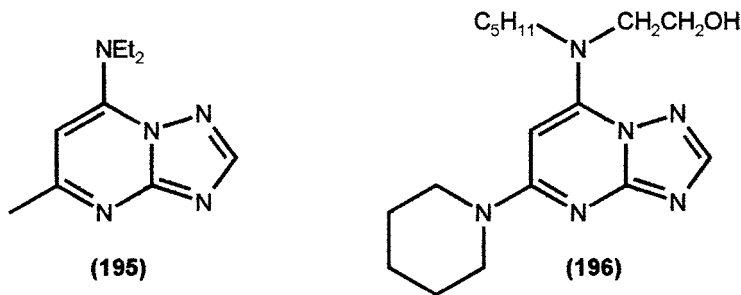
Scheme 50
