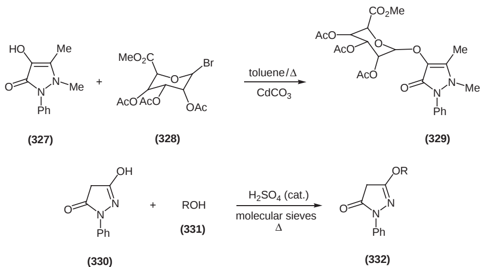
Scheme 89
