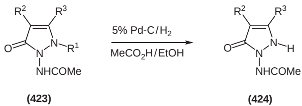
Scheme 116
