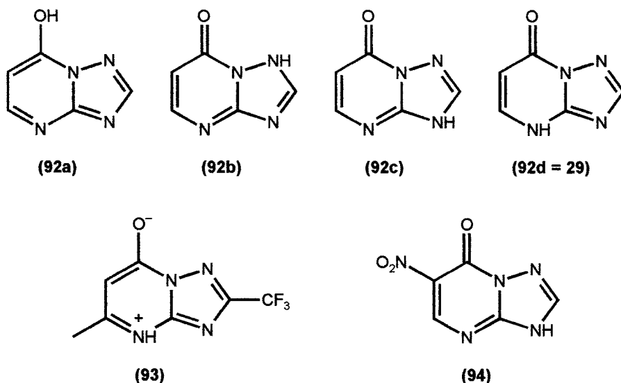
Scheme 24
